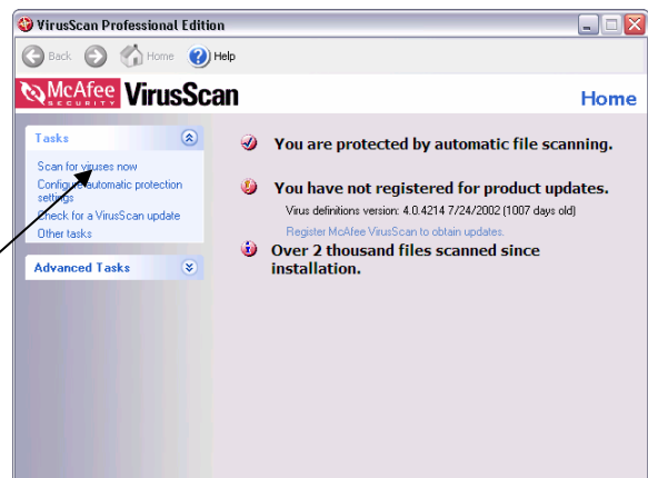
Gambar 20. Scan Virus
